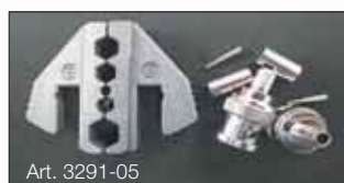
Art. 3291-05 Coaxial RG 58.59.62.6. 6.48 / 5.41 / 2.5 / 1.72 / 8.23 mm 2 0.255 / 0.213 / 0.1 / 0.68 / 0.324"
